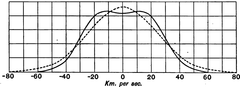
FIG. 18.—Comparison of Two-drift and Ellipsoidal Hypotheses.
